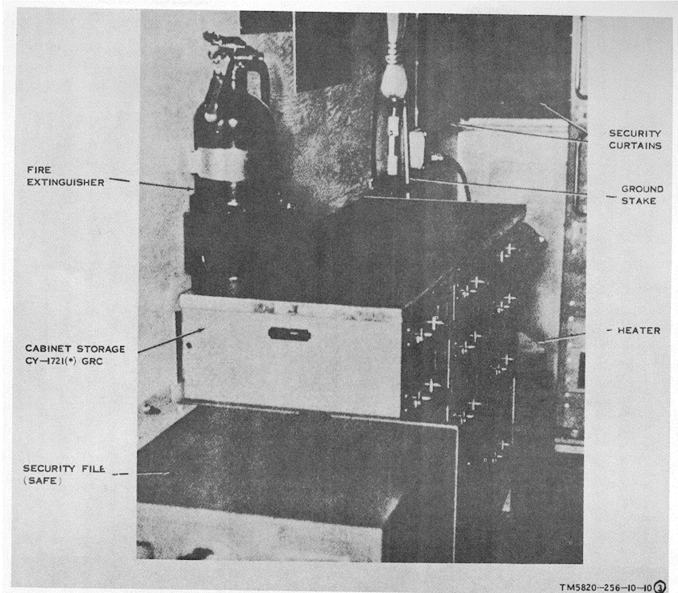
Figure 1-7. Radio Set AN/GRC-26D, interior roadside view from rear door (modified per MWO 11-5820-256-5/1)
