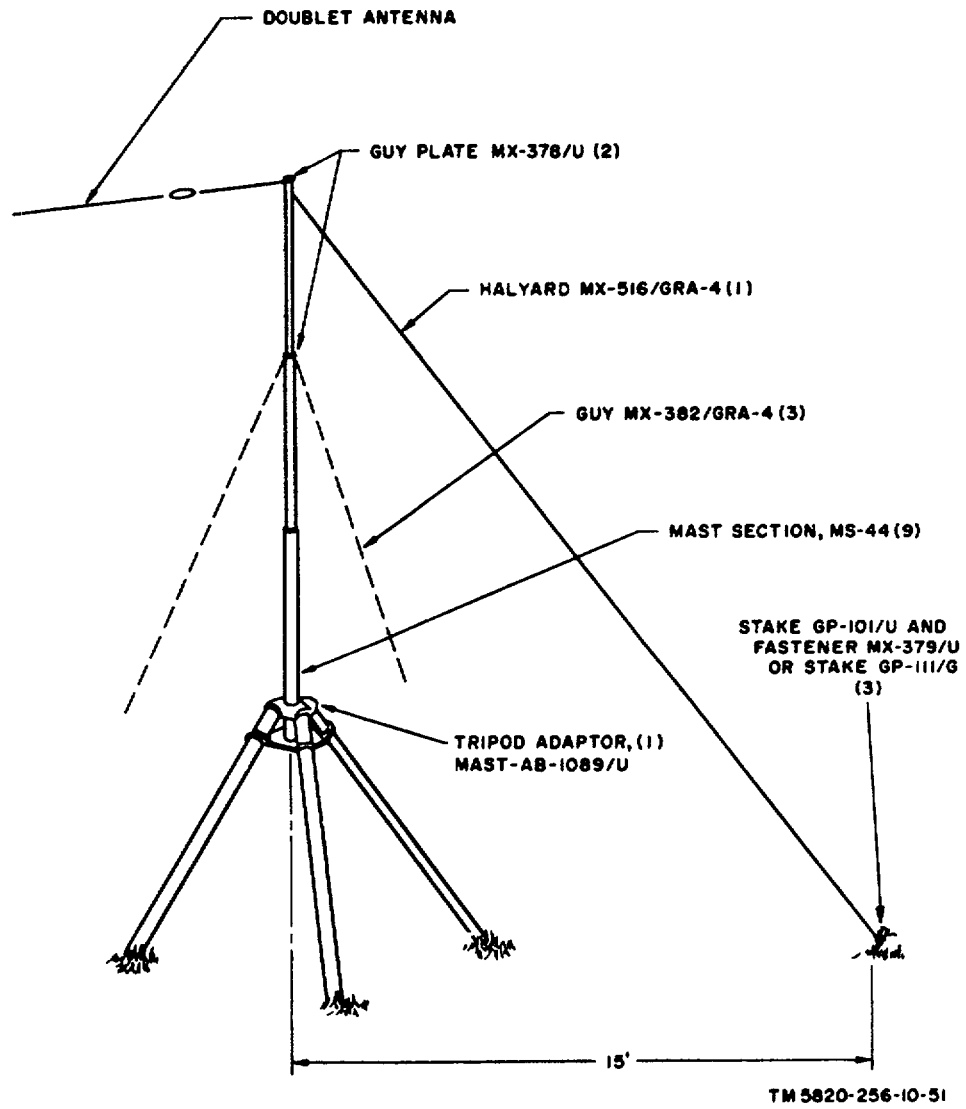
Figure 2-11. Tripod Mast, Typical Installation
