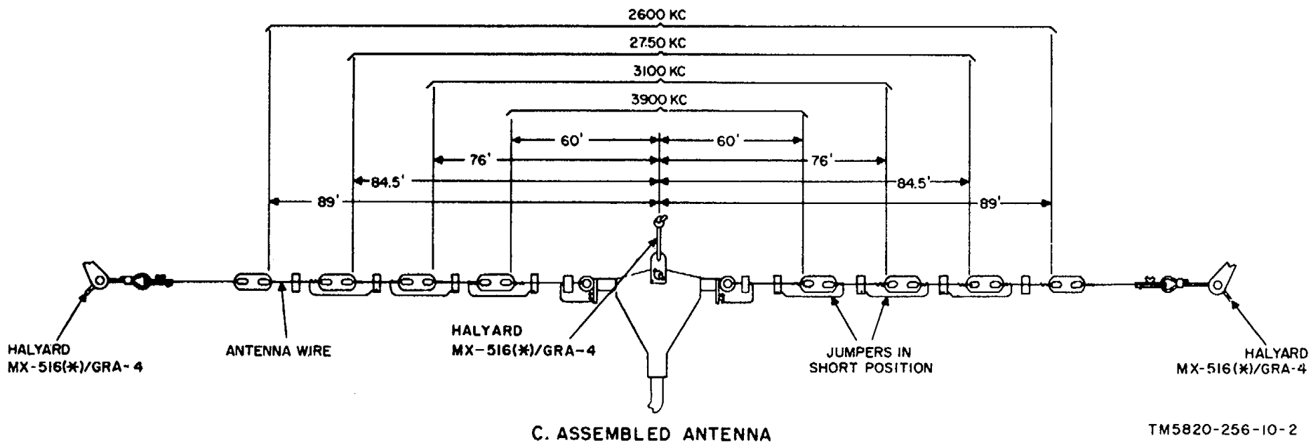
Figure 2-1. Construction and assembly of doublet antenna.
